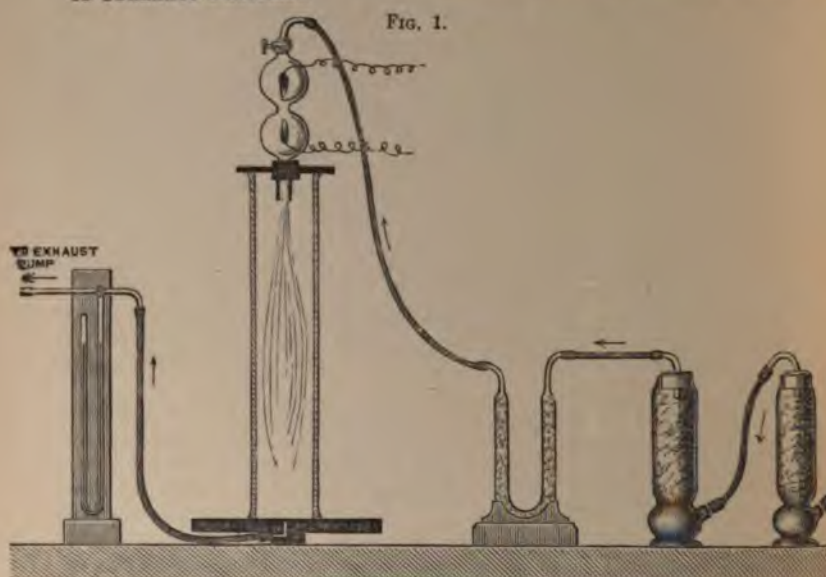
Phosphorescent Gases Apparatus.
